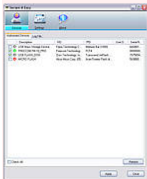
Screenshot Devices
